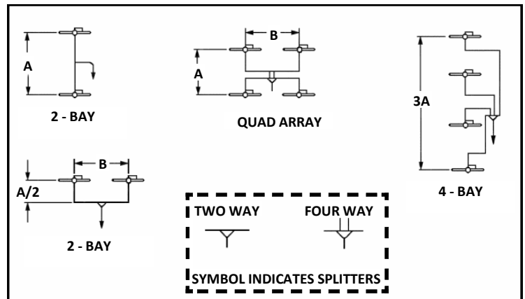
Figure 5: Array Spacing of "J-Series" UHF
